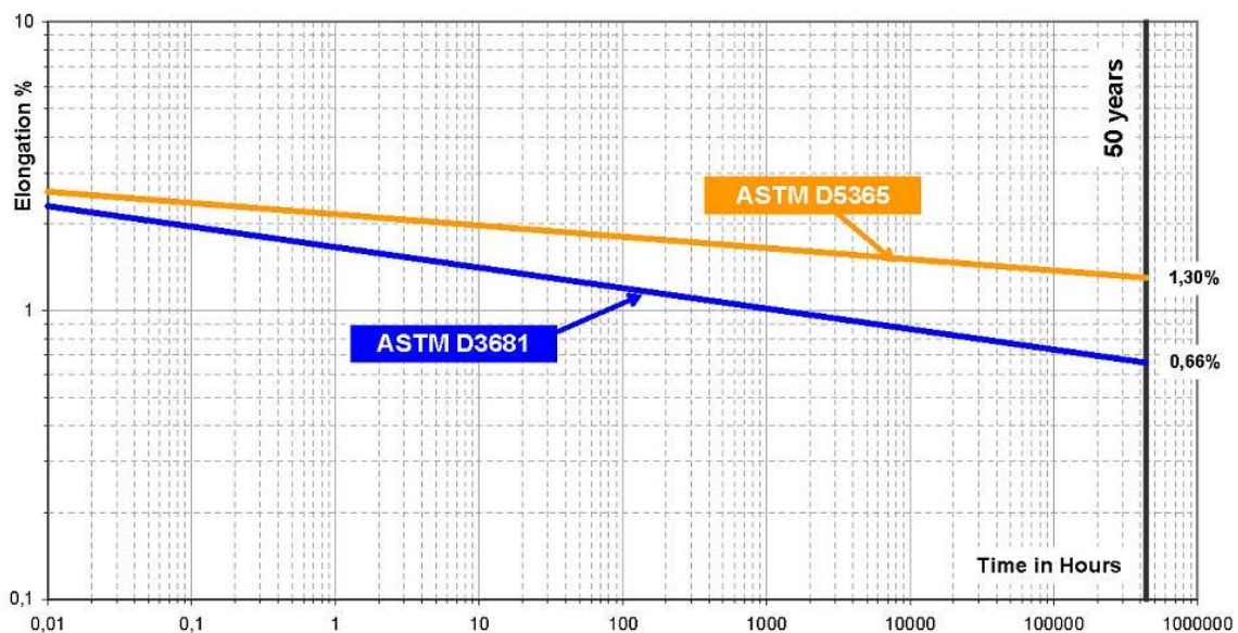
CDB - Strain corrosion of sanitation pipes
